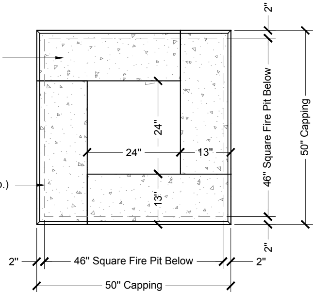
2nd Course Capping Plan
